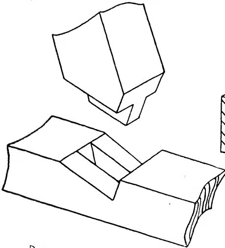
BEVEL-SHOULDER JOINT
